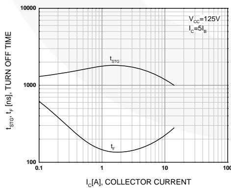
Figure 5. Turn-Off Time
